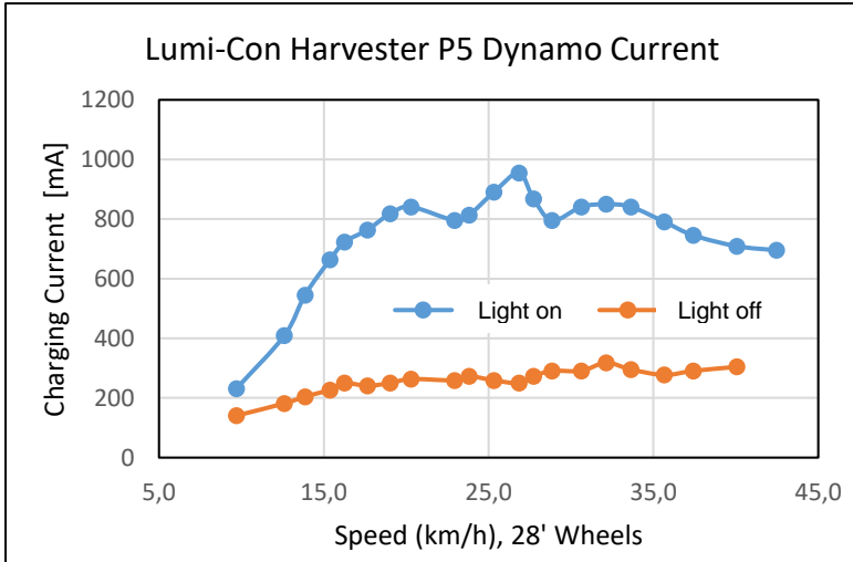
Fig. 3: Charge current and power at a battery voltage of 8V vs. speed, typical hub dynamo (Shimano)
